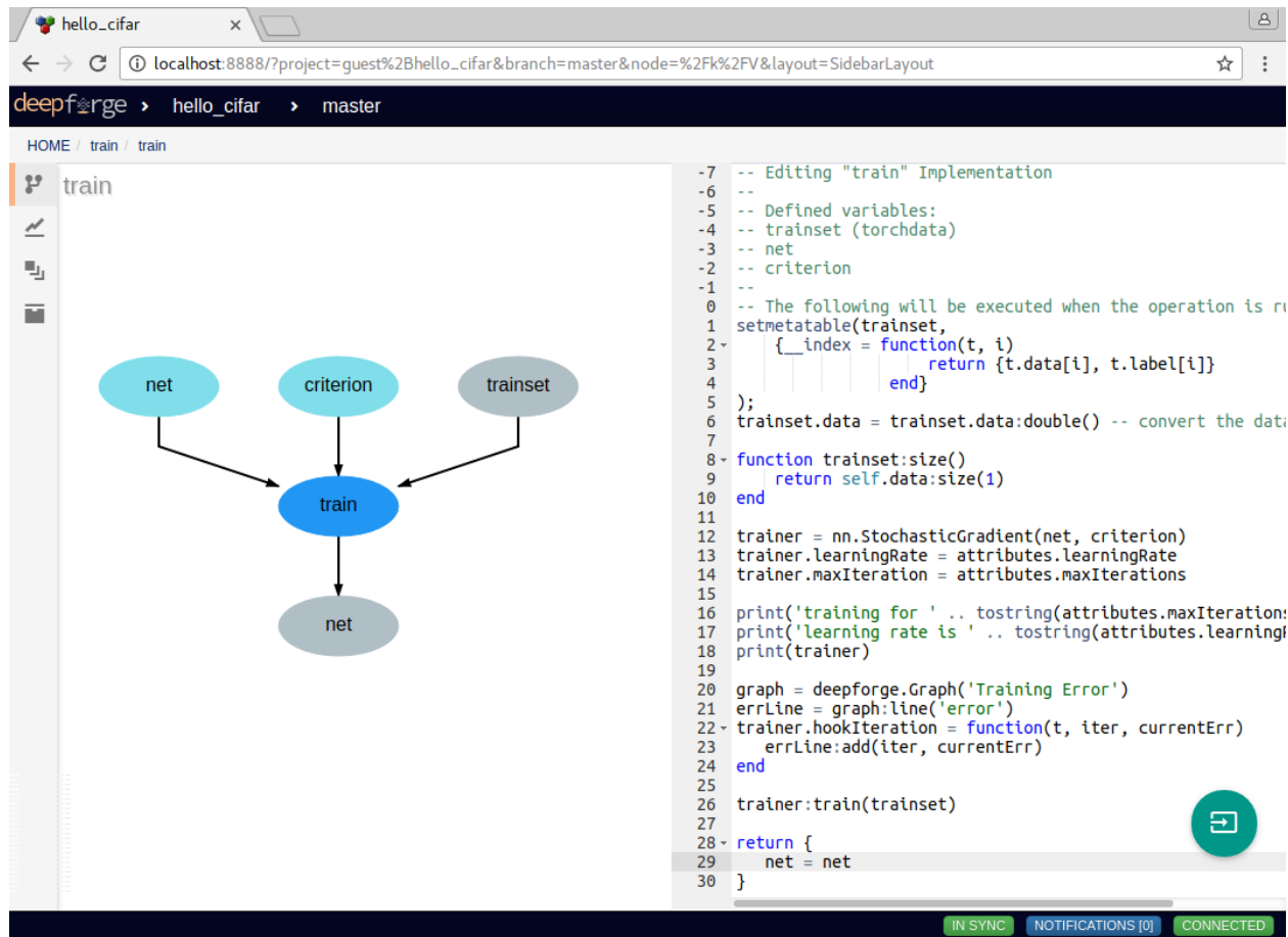
Fig. 1: Editing the “train” operation provided in the “First Steps” section
